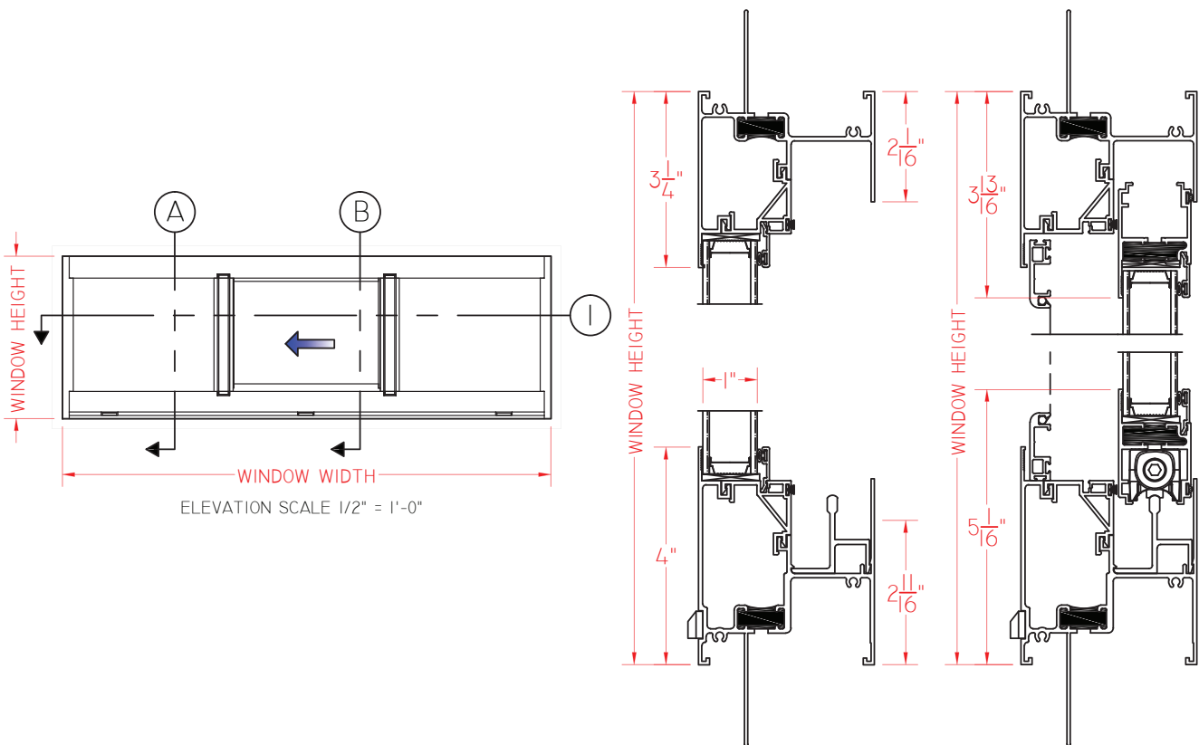
① A VERTICAL CROSS SECTION
