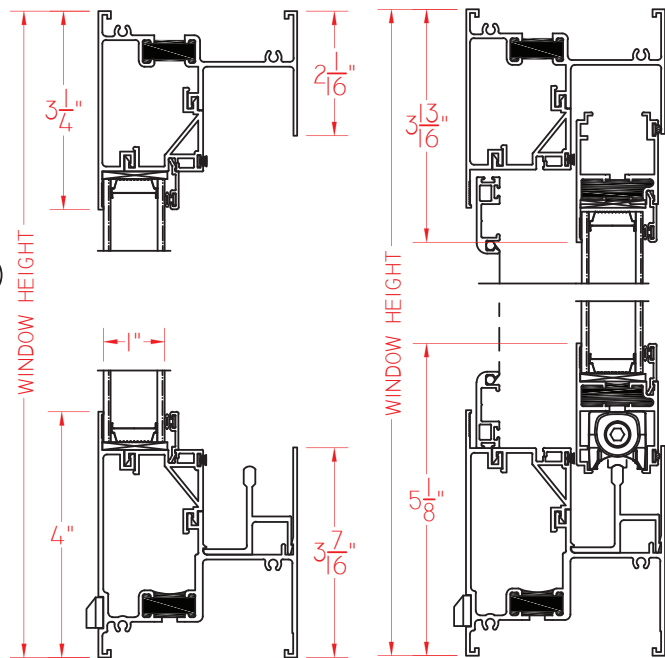
④ A VERTICAL CROSS SECTION
